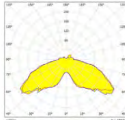
Luminance Distribution
